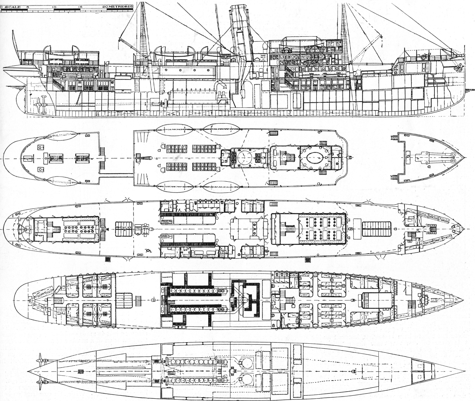
PLANS OF THE "V. PUCHOL" AFTER CONVERSION.
